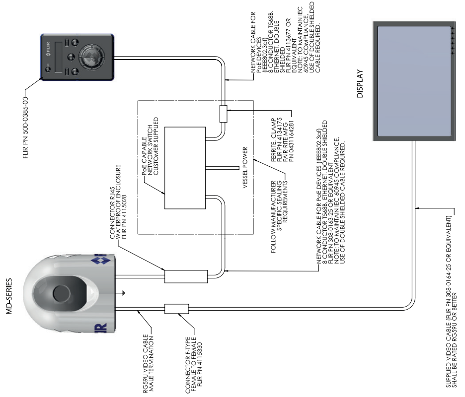
JCU CONTROL - POE SWITCH
